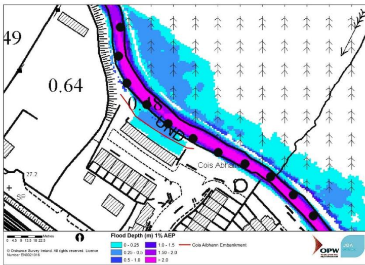
Figure 6-1: Cois Abhainn Embankment Location (UoM 32, 33 Preliminary Options Report)
