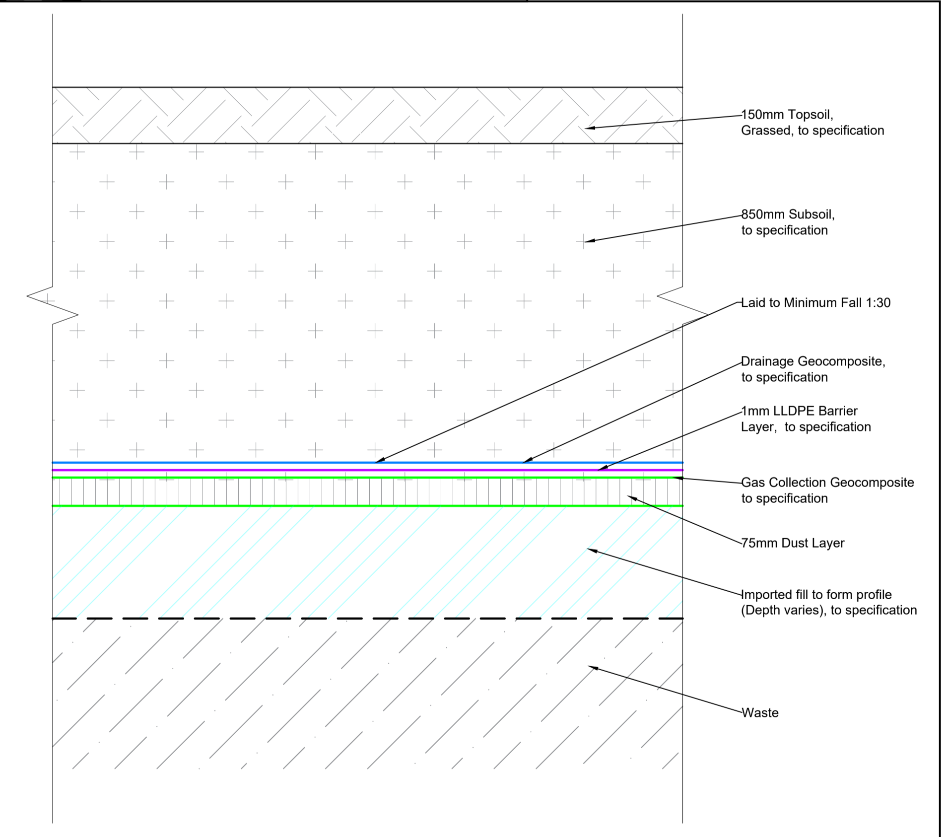
TYPICAL CAPPING DETAIL Scale 1:10
