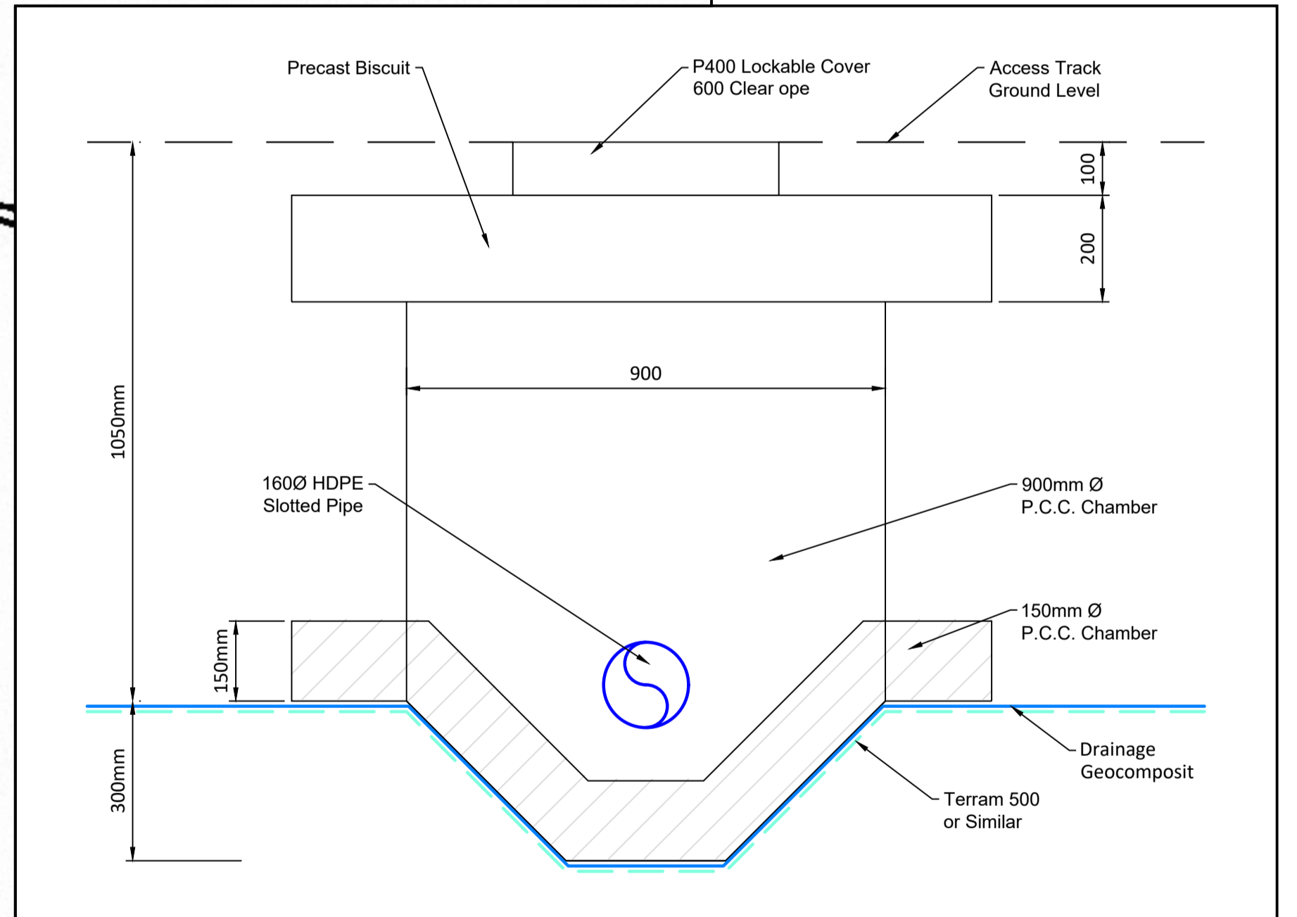
TYPICAL MANHOLE DETAIL Scale 1:10
